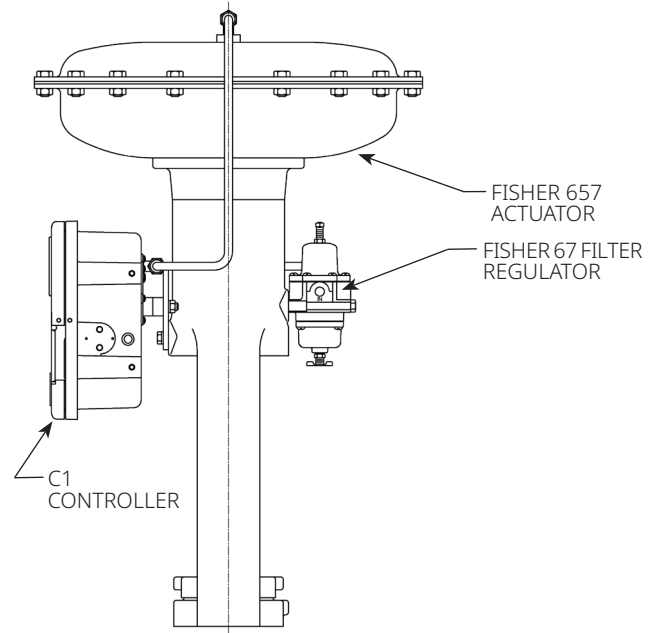
Figure 9. Typical Yoke Mounting
