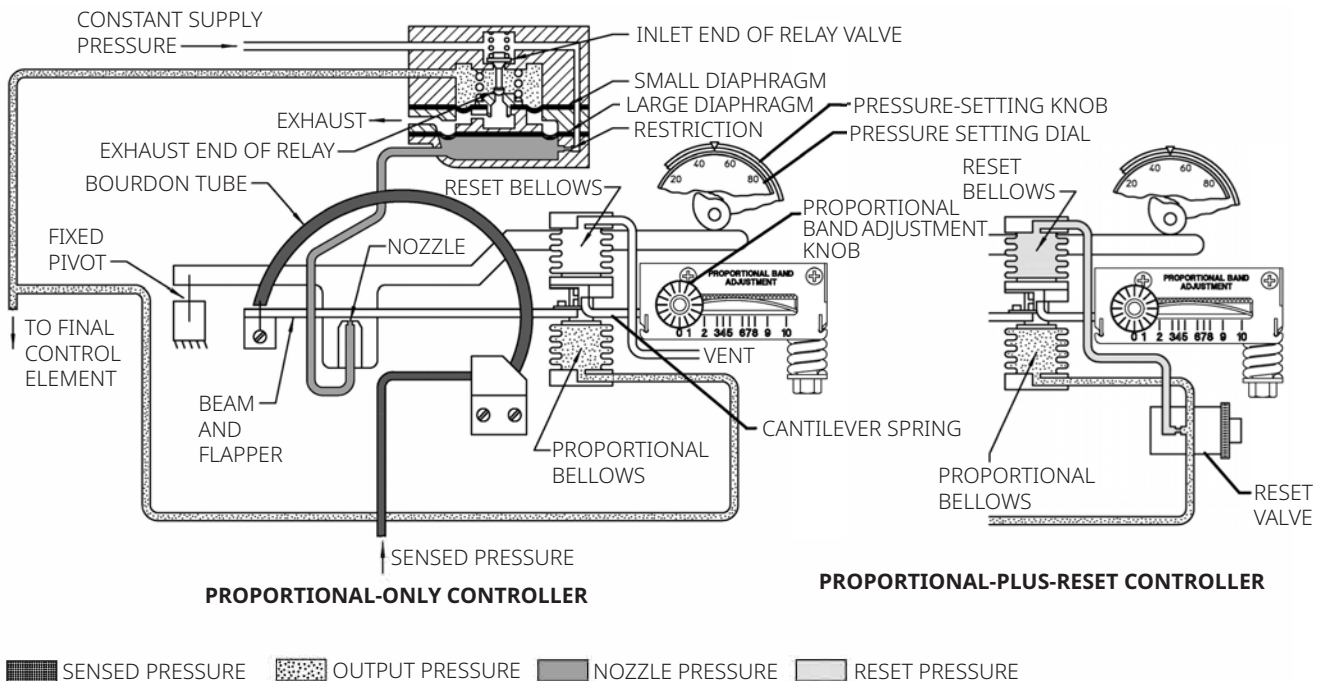
Figure 2. Schematic of Reverse-Acting Proportional-Only and Proportional-Plus-Reset Controllers
