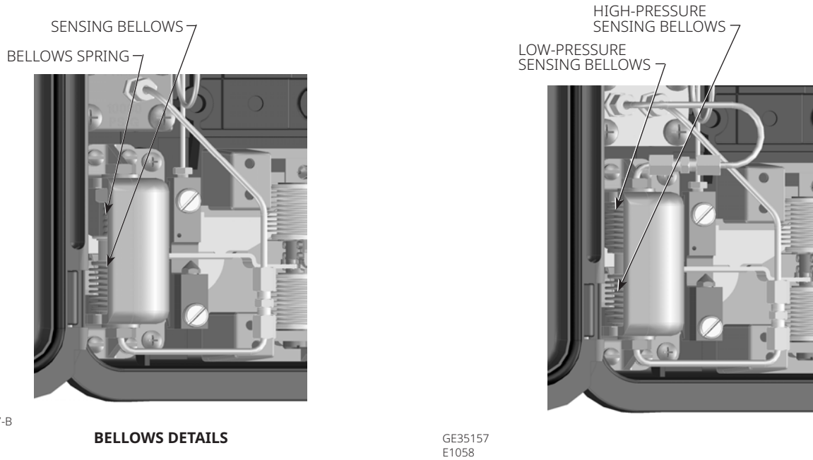
Figure 6. Bellows Details
