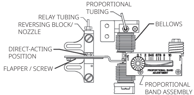
Figure 4. Conversion from Reverse to Direct Action or Proportional to Differential Gap
