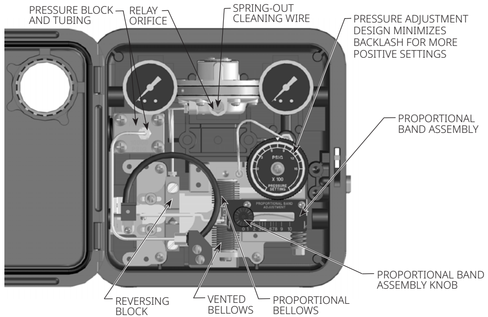
REVERSE-ACTING CONTROLLER PROPORTIONAL
