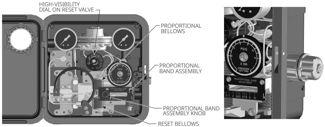
ANTI-RESET WINDUP ASSEMBLY DETAIL
