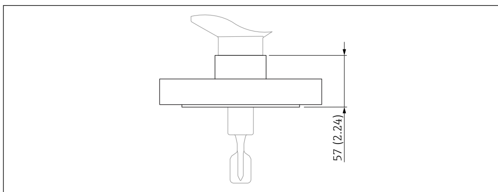
44 Process connection with flange (maximum specification of height) . Unit of measurement mm (in)
