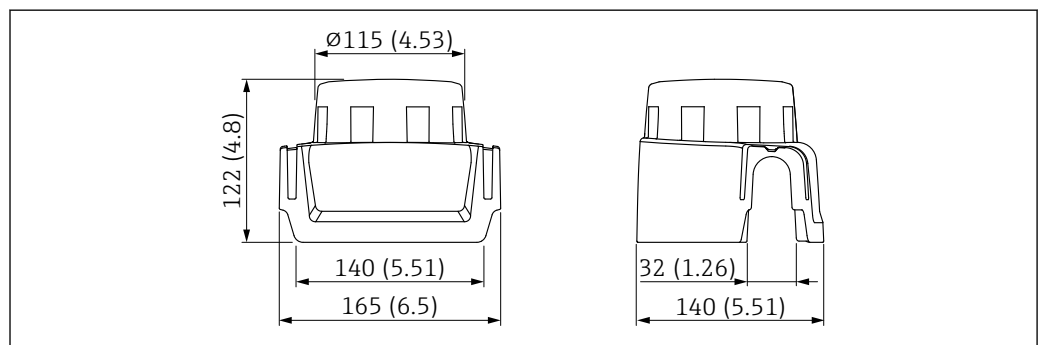
53 Dimensions of protective cover, plastic, XW111. Unit of measurement mm (in)
