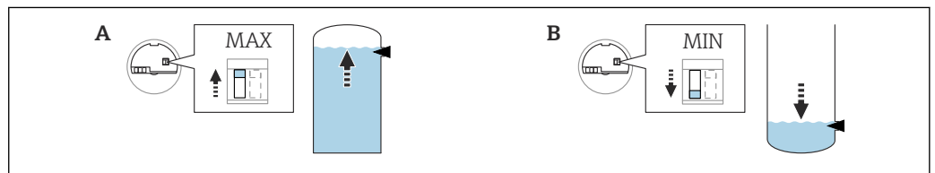
46 Switch position on the electronic insert for MAX/MIN safety mode
