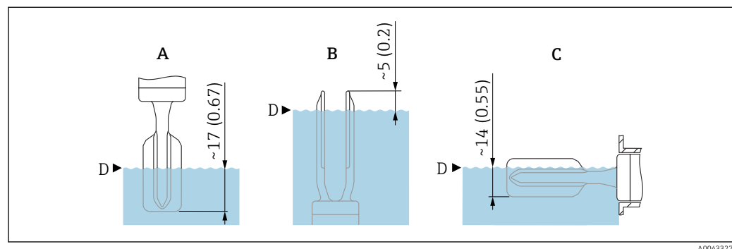
18 Typical switch points, enamel-coated vibrating fork, dimensions without coating thickness. Unit of measurement mm (in)
