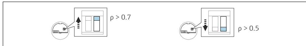
47 Switch position on the electronic insert for density
