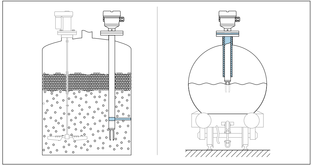
31 Examples of support in the event of dynamic load
