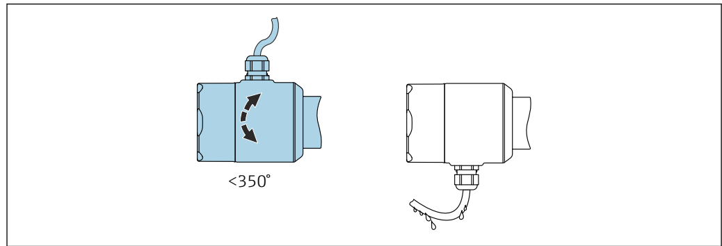
28 Housing without locking screw with drip loop
