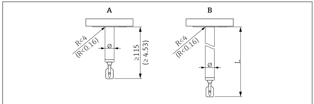
41 Probe design: short pipe, pipe extension. Unit of measurement mm (in)
