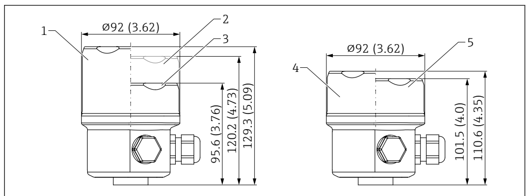
38 Dimensions of single-compartment housing, 316L, hygienic. Unit of measurement mm (in)
