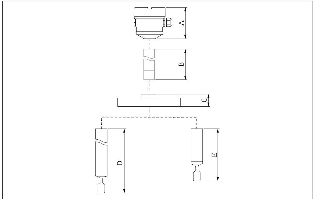
33 Components to determine the device height
