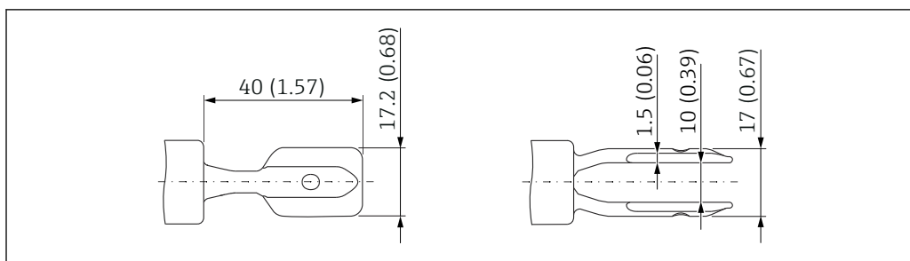
42 Tuning fork with plastic coating (ECTFE, PFA). Unit of measurement mm (in)
