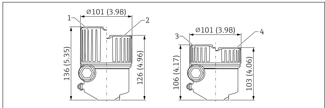
▣ 35 Dimensions of single-compartment housing, aluminum, coated. Unit of measurement mm (in)
