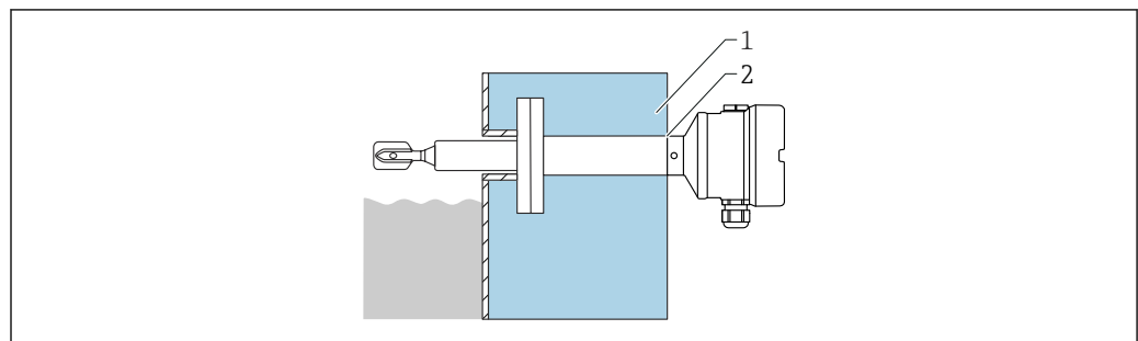
30 Vessel with heat insulation (example with temperature spacer)
