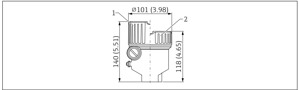
36 Dimensions of single compartment housing, aluminum, coated; with Ex d/XP, dust ignition-proof. Unit of measurement mm (in)
