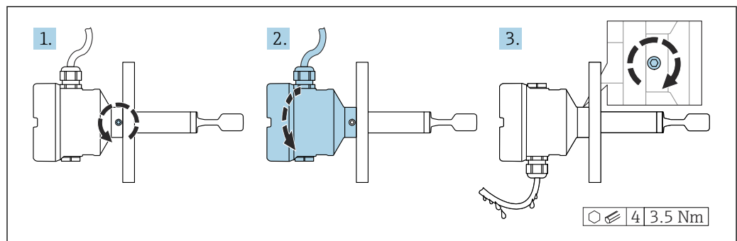
29 Housing with external locking screw and drip loop
