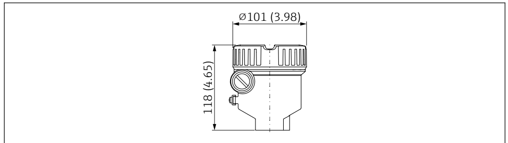
37 Dimensions of single compartment 316L housing; with Ex d/XP also, dust ignition-proof; cover without sight glass. Unit of measurement mm (in)
