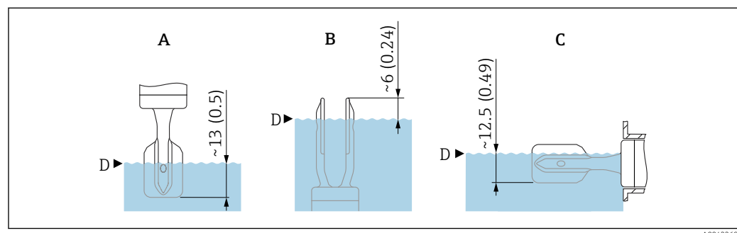
17 Typical switch points, plastic-coated vibrating fork (ECTFE, PFA), dimensions without coating thickness. Unit of measurement mm (in)
