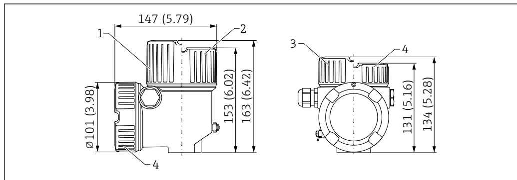
39 Dimensions of dual compartment housing, L-shaped, aluminum, coated; also with Ex d/XP, dust ignition-proof. Unit of measurement mm (in)
