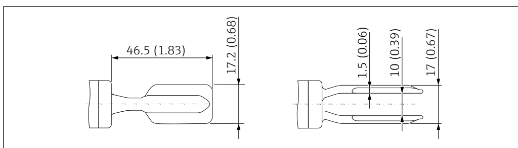
43 Tuning fork with enamel coating. Unit of measurement mm (in)
