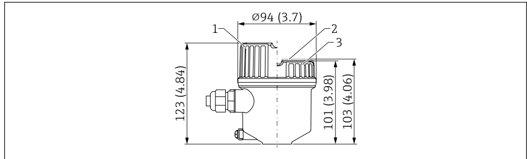
▣ 34 Dimensions of single compartment housing, plastic. Unit of measurement mm (in)
