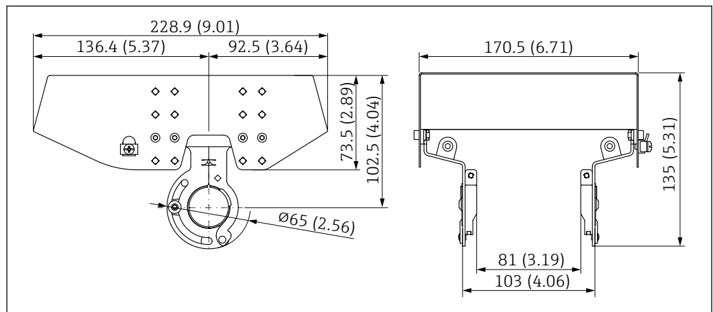
52 Dimensions of protective cover, 316 L, XW112. Unit of measurement mm (in)
