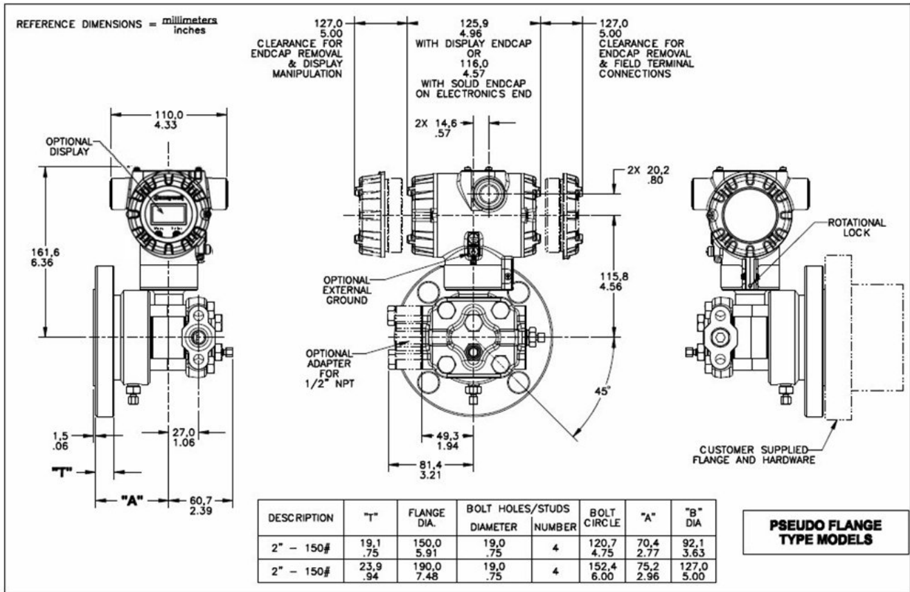
Figure 6 – Typical mounting dimensions for pseudo flange type models STF72P and STF73P
