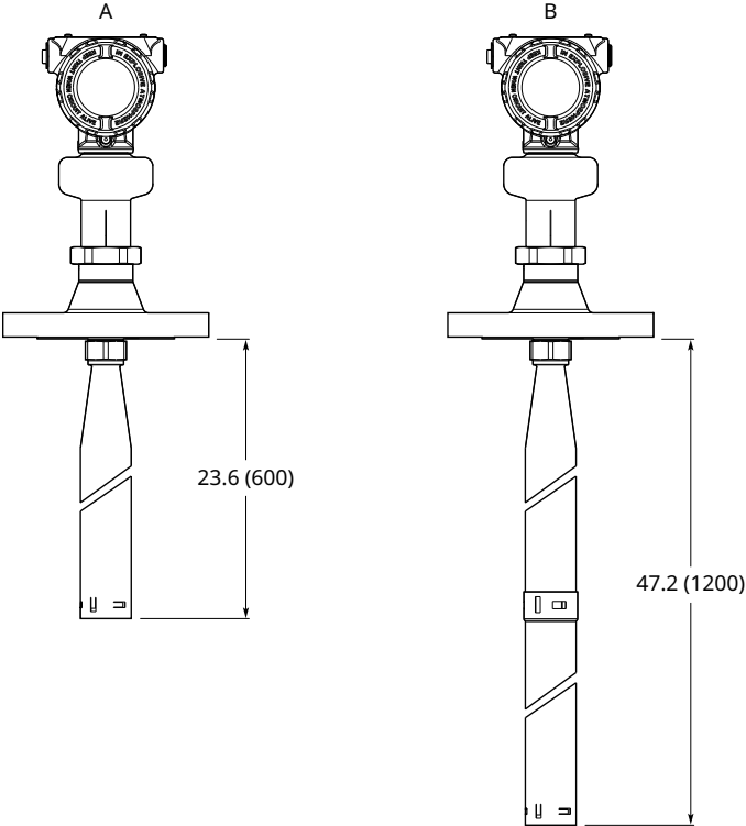
Figure 27: Extended Cone Antenna
