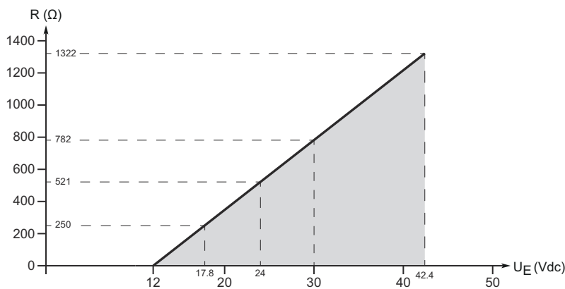
Figure 3: Load Limits
