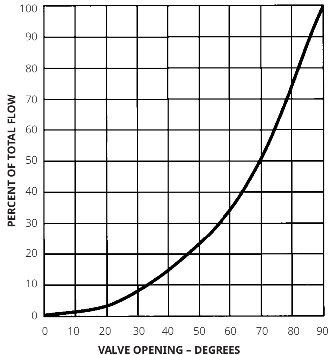
Figure 5. Severe Service Trim Valve Characteristics
