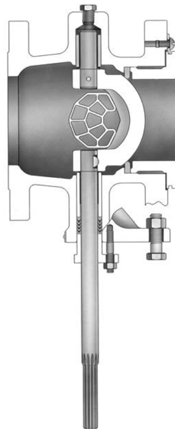
Figure 7. Fisher Vee-Ball Series Rotary Attenuator Construction
