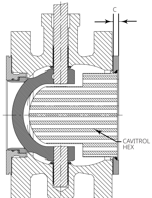
Figure 9. Fisher NPS 8 V300 Cavitrol Hex Cross Sectional View
