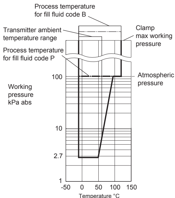
Figure 1i. Working Pressure and Process Temperature (Fill fluid: silicone oil)
